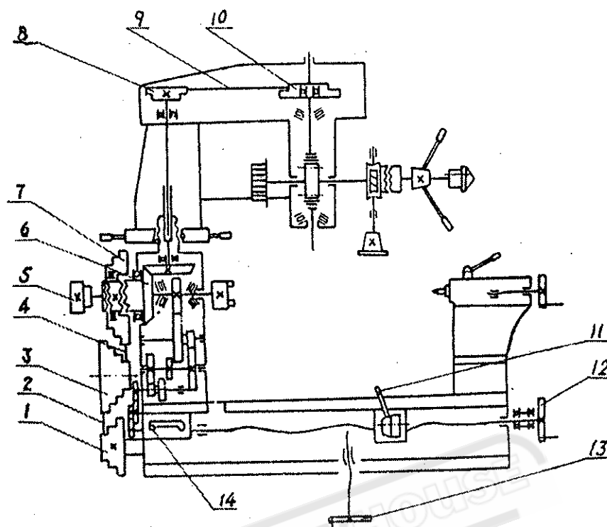
Fig.5 Transmission system
